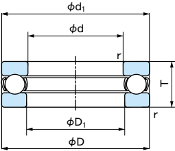
Flat back-face type
