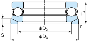
With aligning seat
