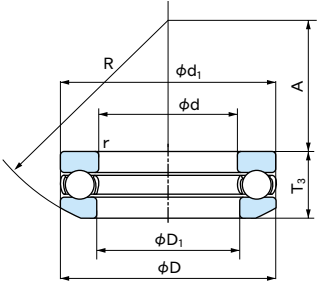
Spherical back-face type
