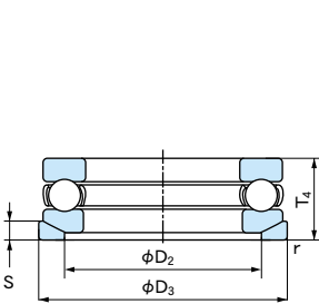
With aligning seat
