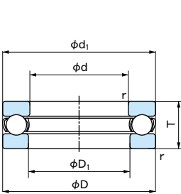
Flat back-face type
