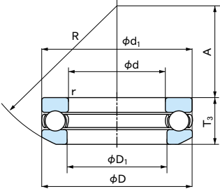
Spherical back-face type
